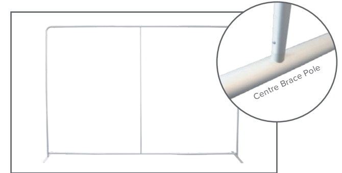
Step 3: Next, clip in the Vertical Brace Pole to the Bottom Horizontal bar before assembling the top of your frame. This makes it easier to assemble the rest of your frame. Continue to match the corresponding numbers on the poles and connect them to build the rest of your frame.
